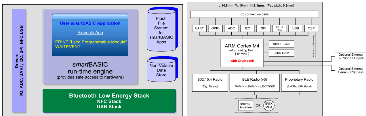
Figure 1: Bluetooth smart BASIC module block diagram
