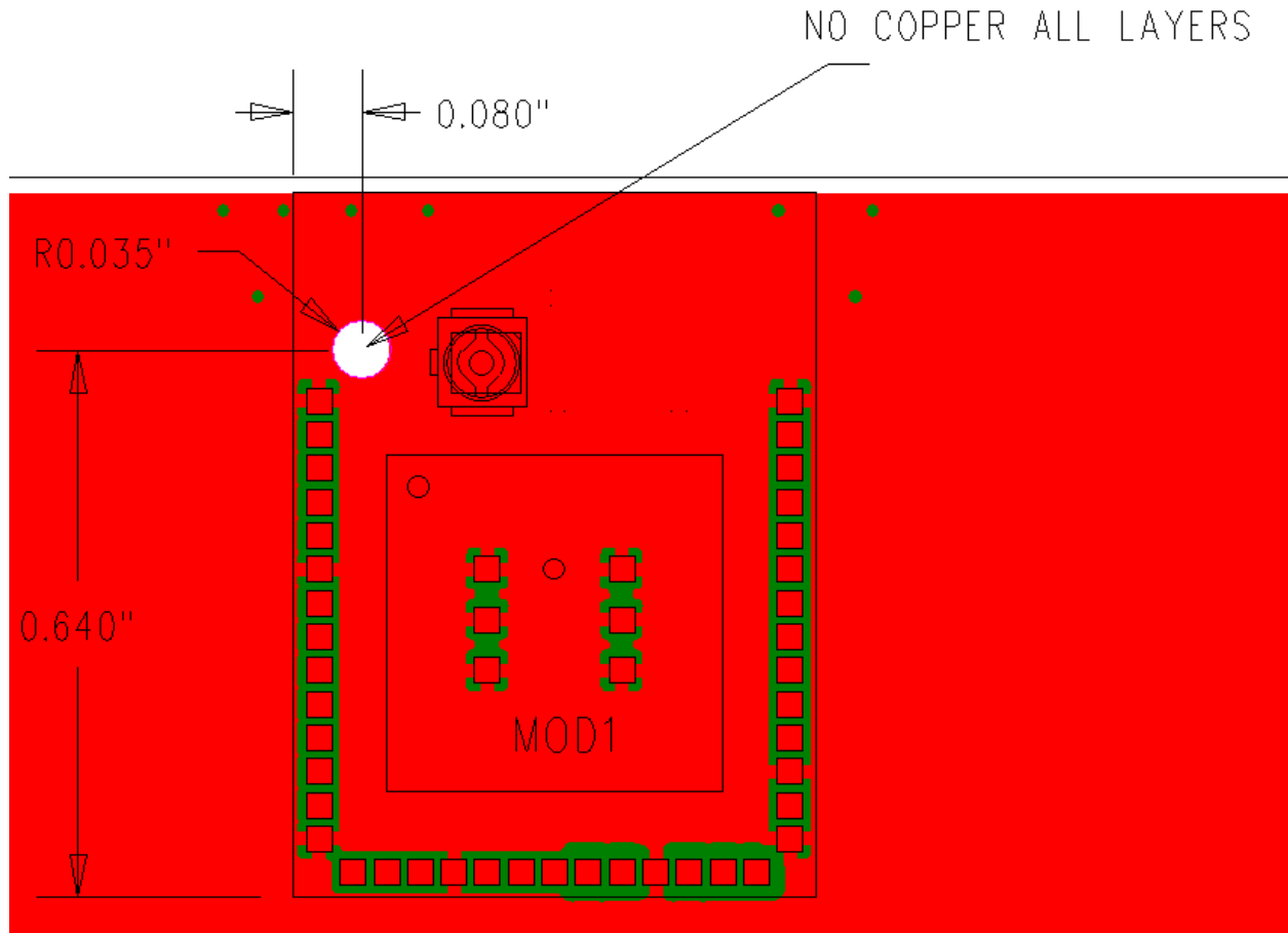
Figure 4 Host PCB for Sterling-LWB U.FL Module Variant
