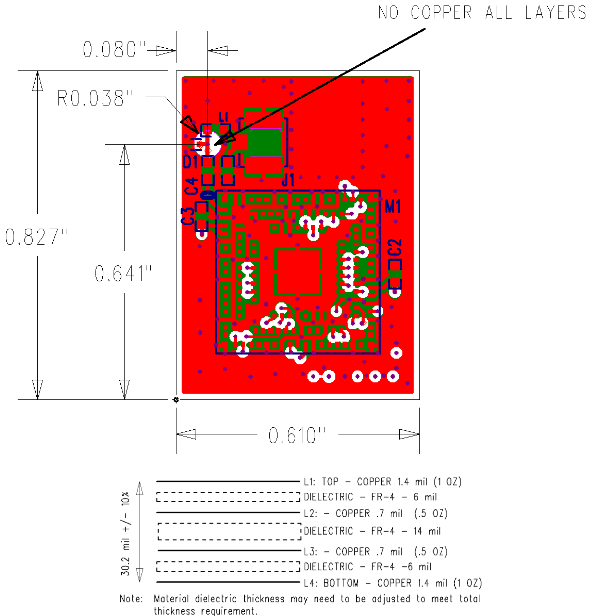
Figure 3 SIP Module with U.FL (External Antenna) Reference Design
