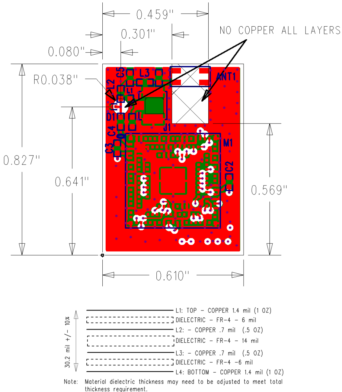
Figure 1 SIP Module with Chip Antenna Reference Design
