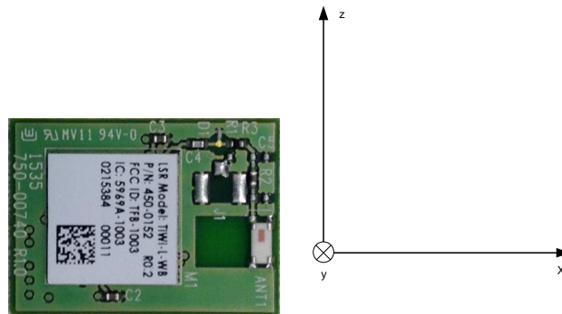
Figure 7 Chip Antenna Typical Radiation Patterns, Orientation Axis shown. 2D-Patterns in standard Spherical Coordinate System ( r, \theta, \phi )
