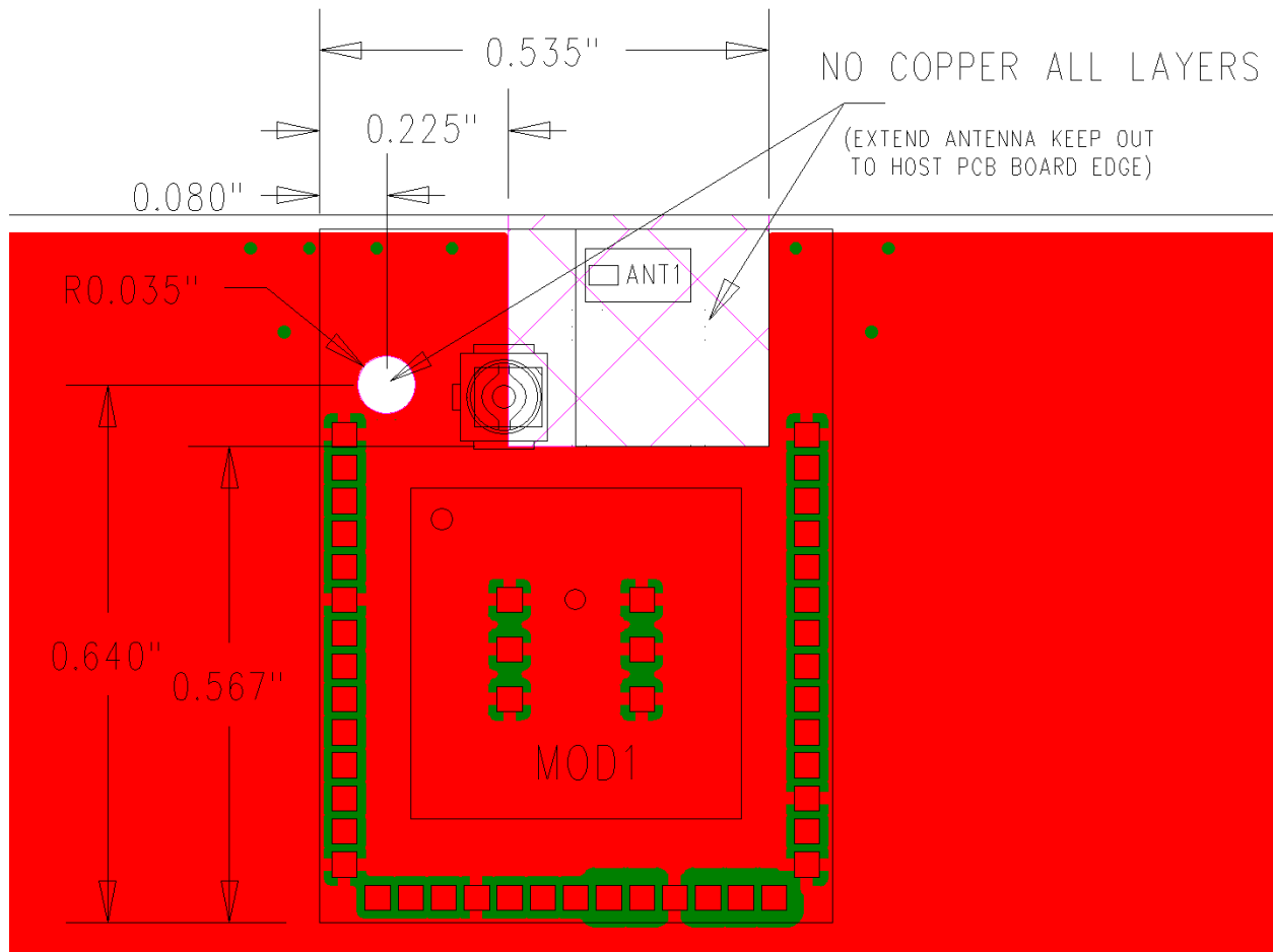
Figure 2 Host PCB for Sterling-LWB Chip Antenna Module Variant
