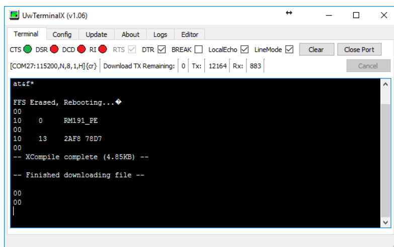
Figure 29: File downloaded
