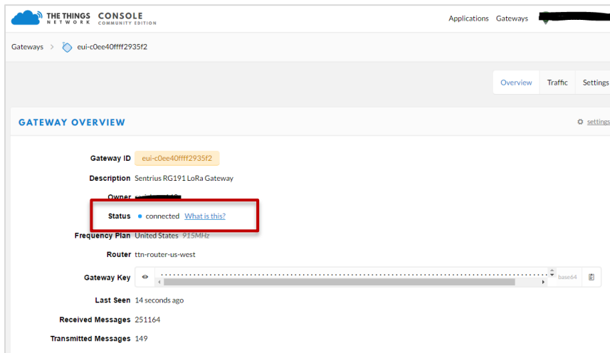
Figure 19: Registered gateway
