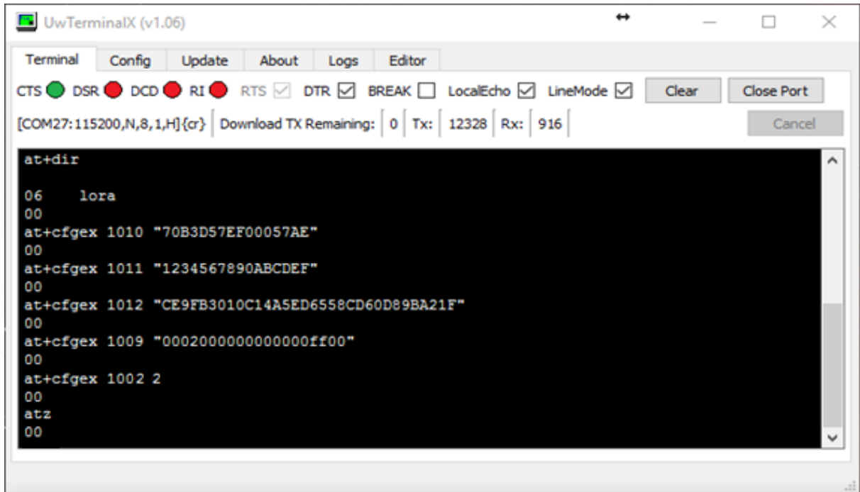
Figure 33: Commands sent
