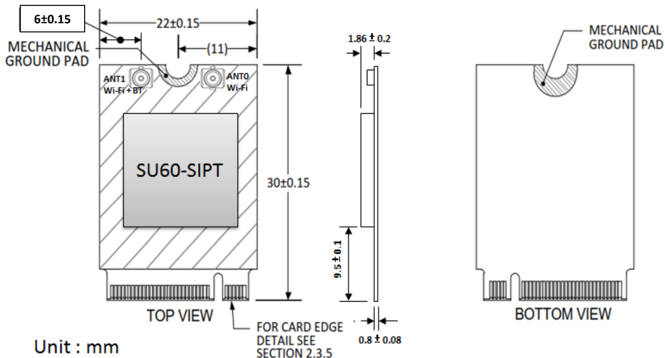
Figure 4: Module dimension of 60-2230C-P/60-2230C-PU
