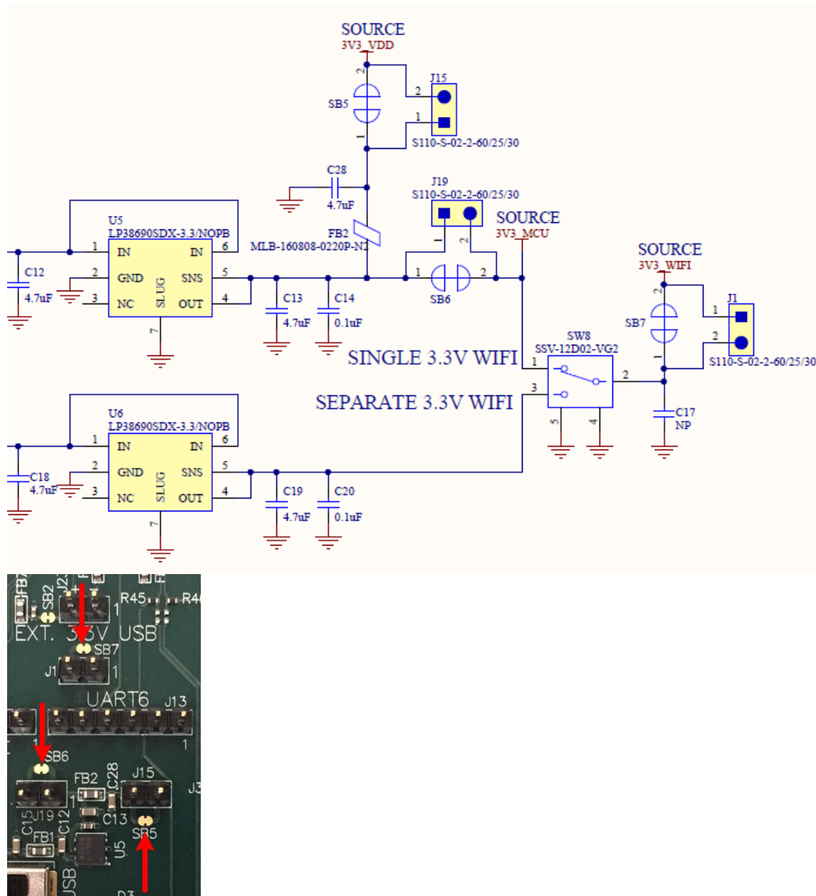
Figure 11: Current measurement schematic and PCB modifications
