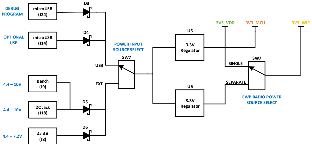
Figure 4: EWB development Kit power supply
