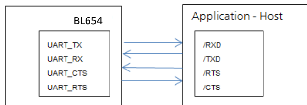
Figure 6: UART signals
