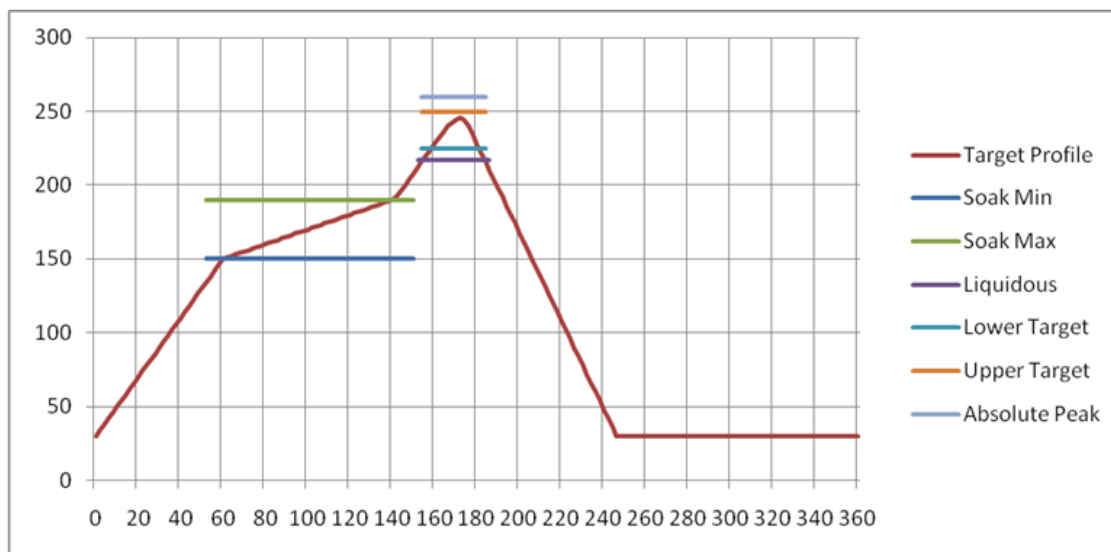
Figure 20: Recommended reflow temperature
