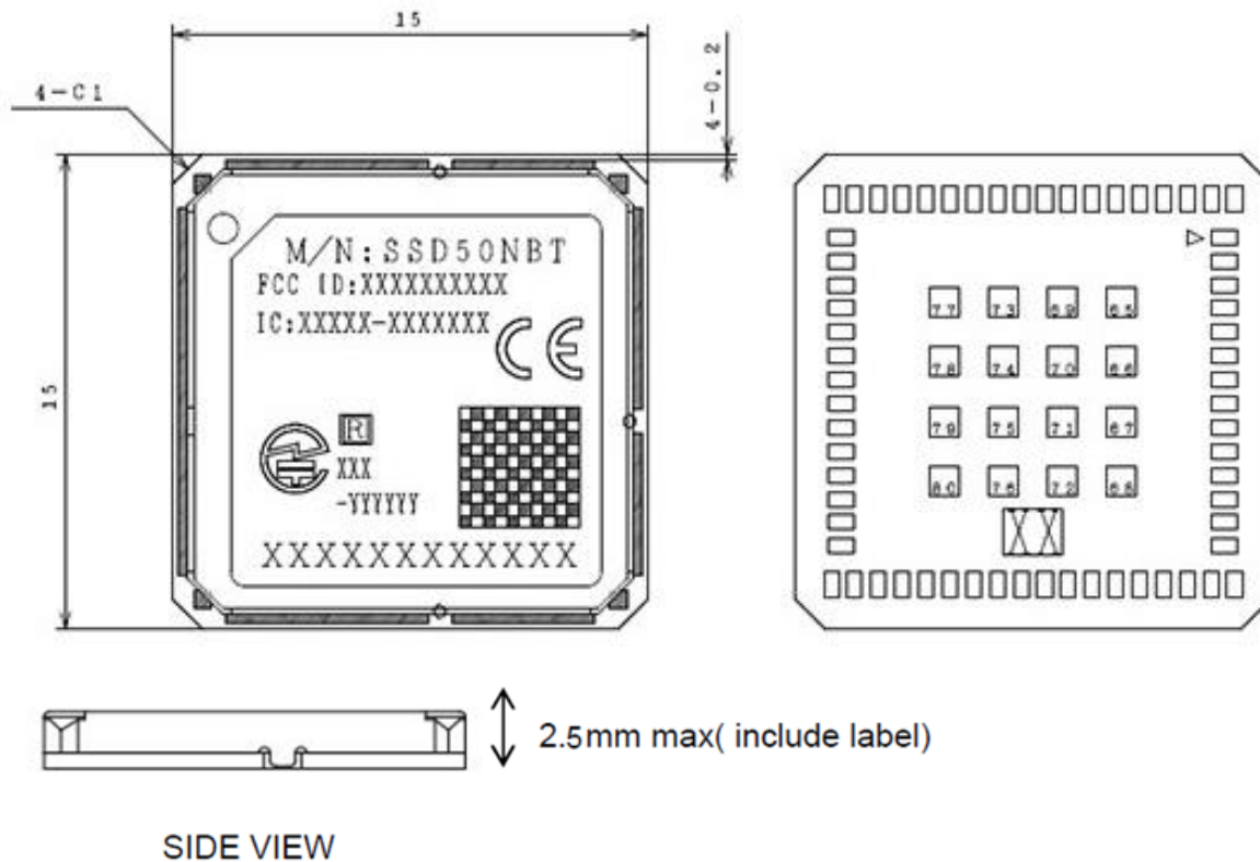
Figure 6: Module dimension of SSD50NBT
