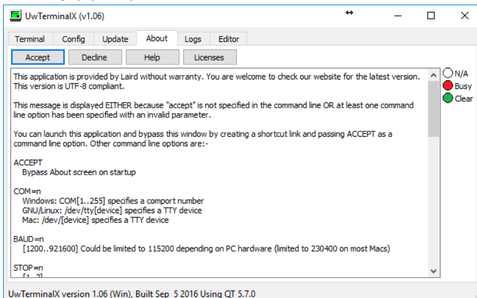
Figure 25: UwTerminalX
