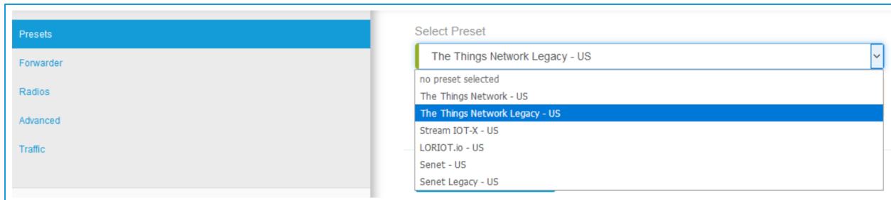
Figure 12: LoRa presets
