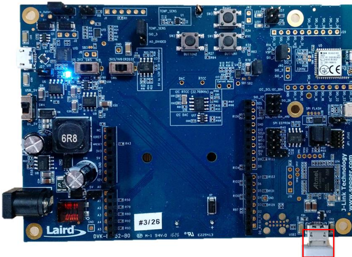
Figure 23: Connecting BL652 to PC through USB2 port
