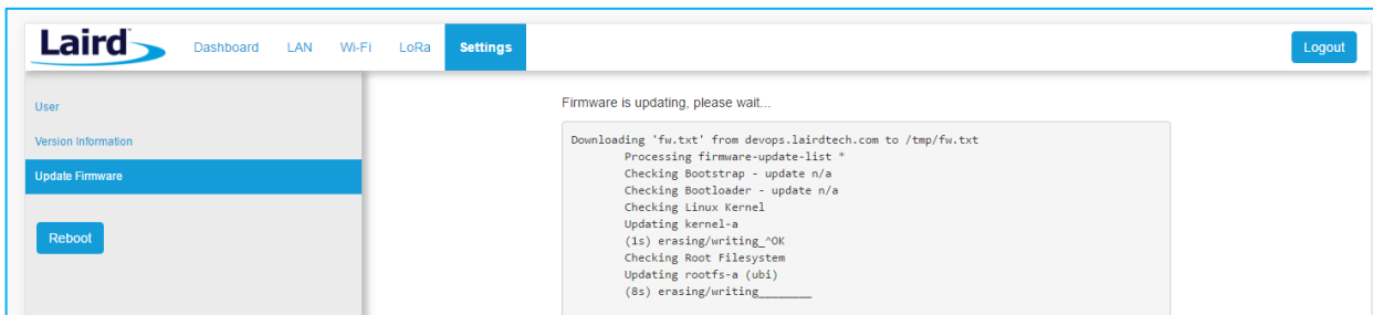
Figure 36: Progress indicator
