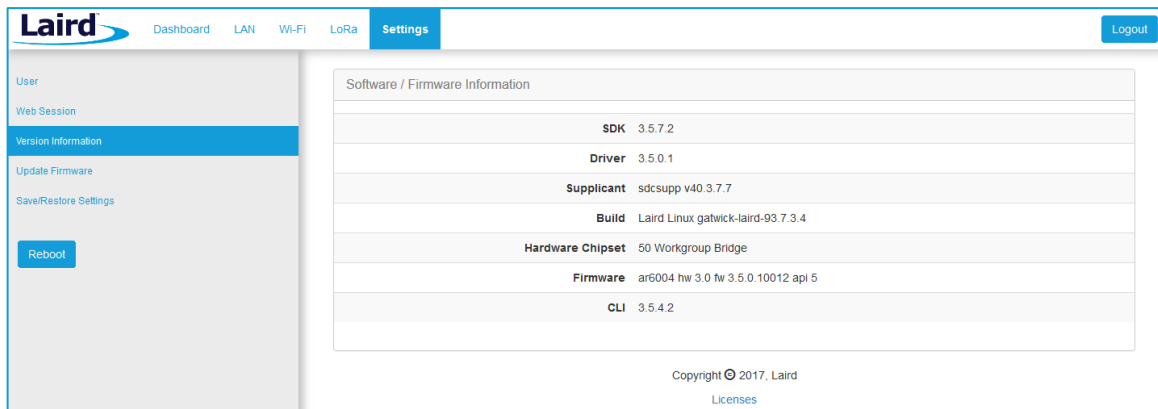
Figure 34: Version information
