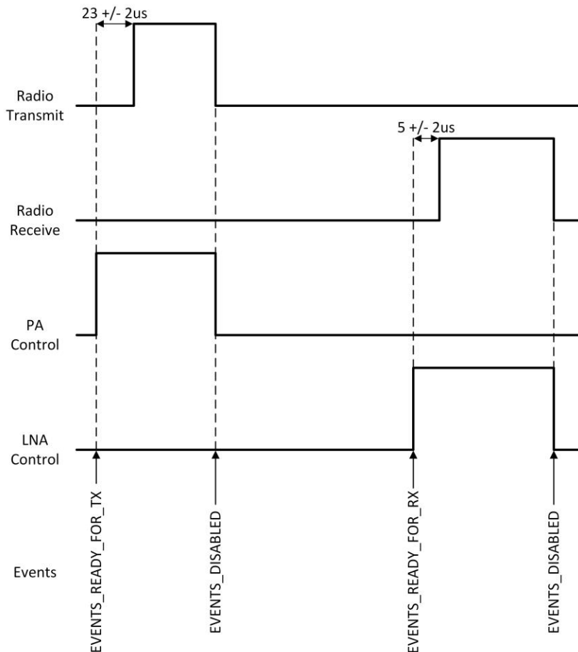
Figure 2: SKY66112 control interface timing and associated events
