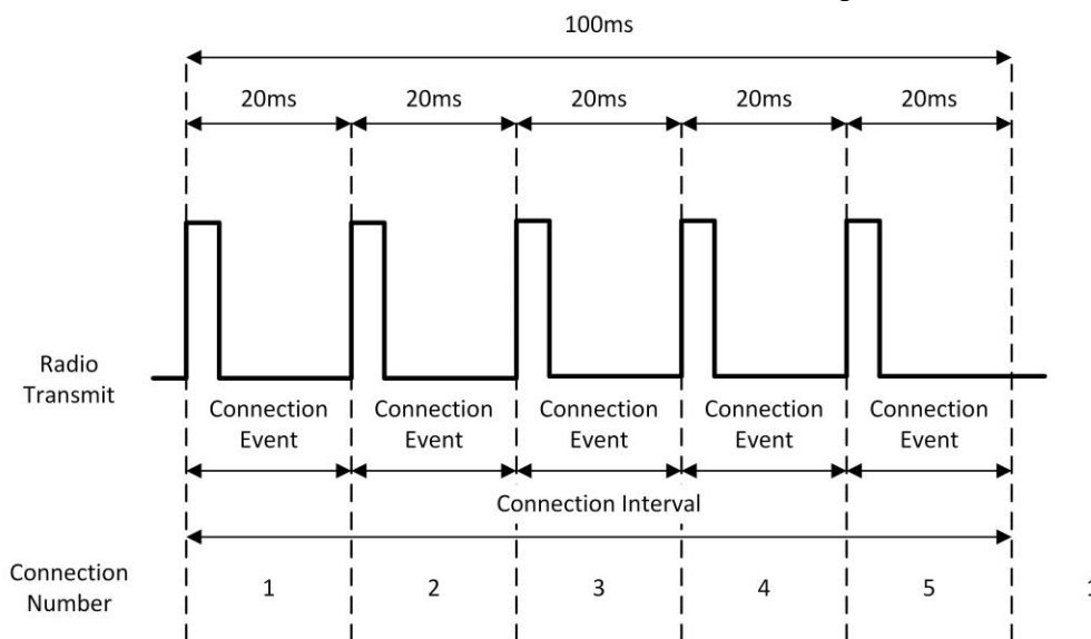
Figure 3: Relationship of connection interval, event length, and number of connections
