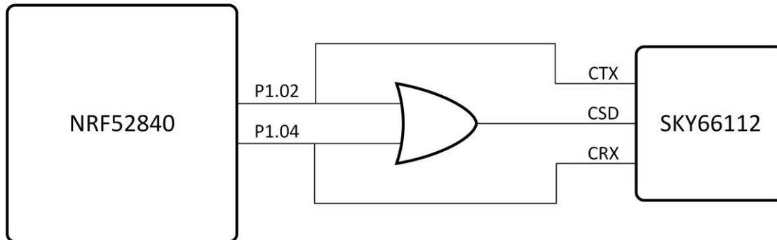
Figure 1: SKY66112 control interface
