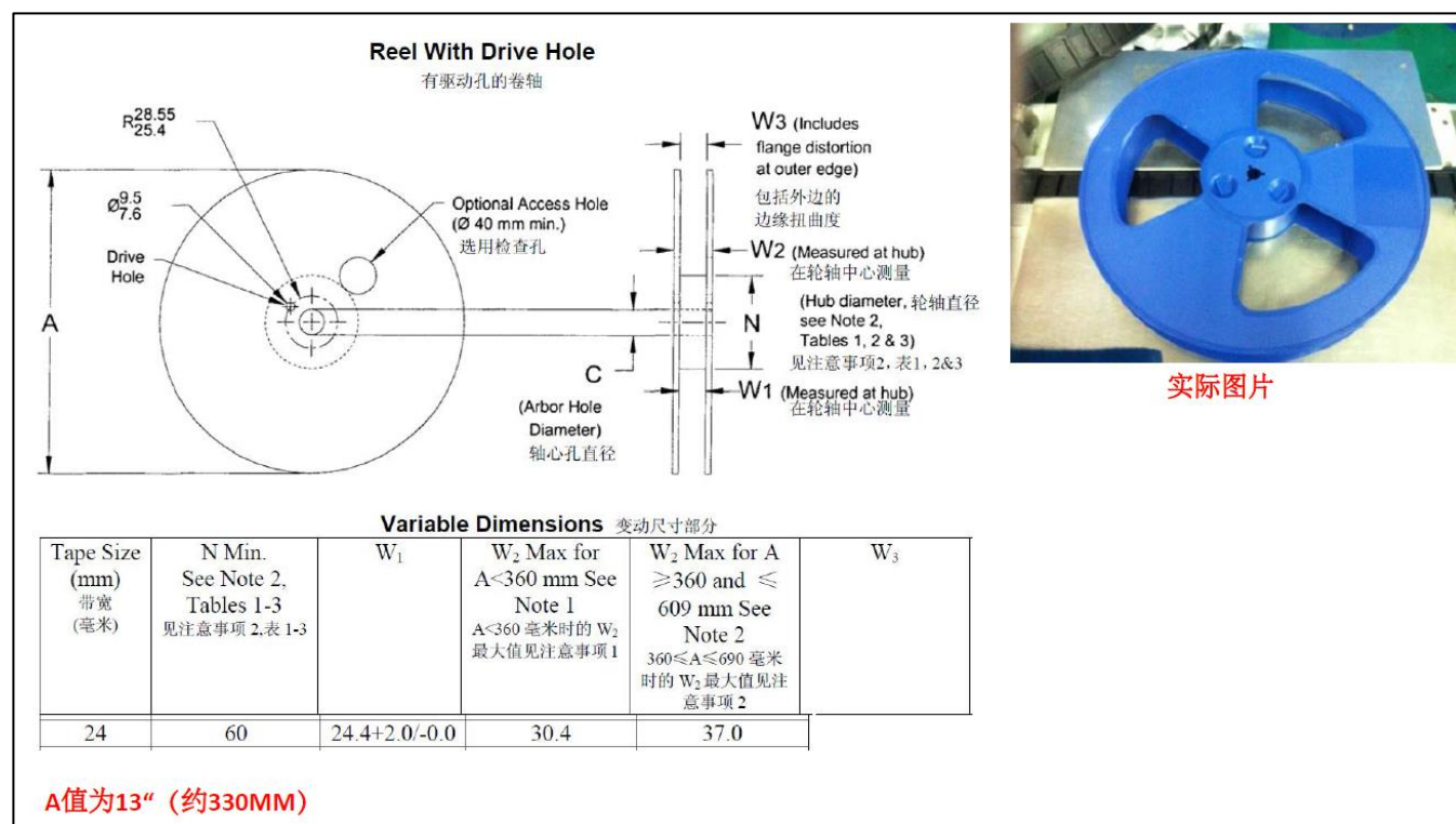
Figure 13: Reel specifications
