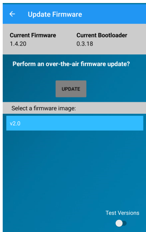
Figure 14: Available update
