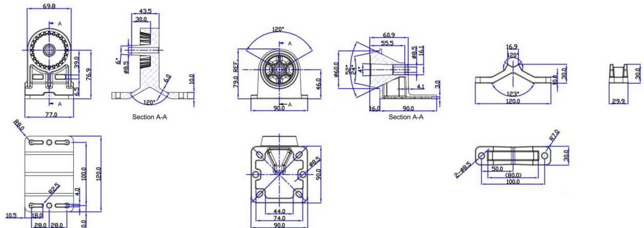
Figure 63: Pole mount dimensions
