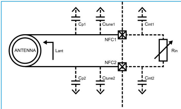
Figure 4: NFC antenna coil tuning capacitors
