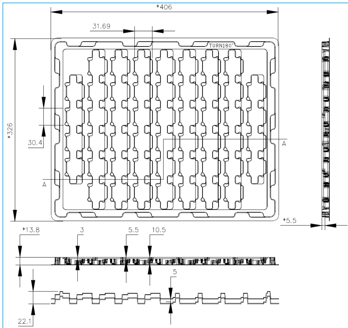
Figure 12: 453-00011 modem tray (mm) 50 per tray
