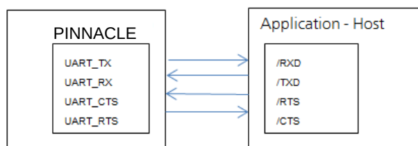
Figure 5: UART signals
