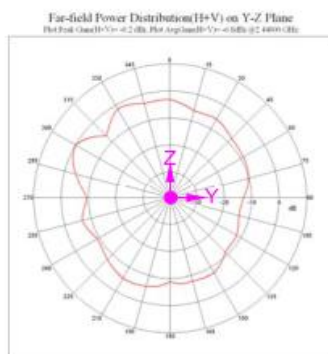
Figure 15: Antenna pattern
