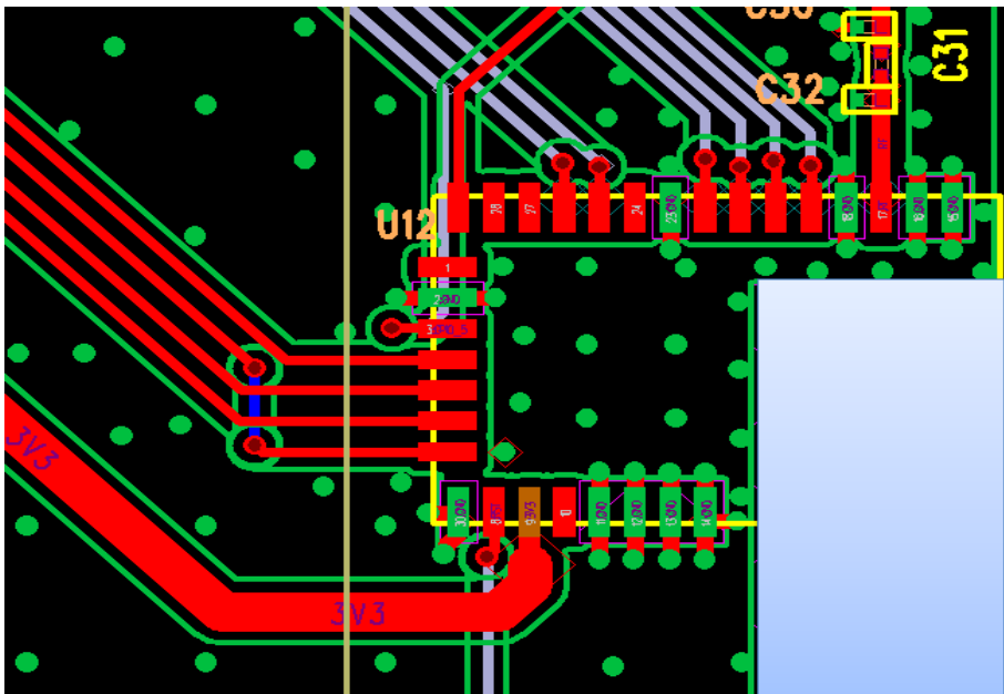
Figure 16: Recommend Antenna keep-out area (in Blue) used on the BT860
