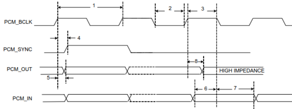
Figure 3: PCM timing diagram (Short-Frame Sync, Master Mode)
