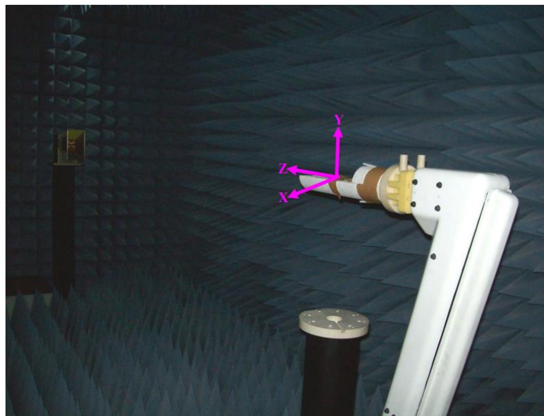
Figure 14: Measurement XYZ polarization
