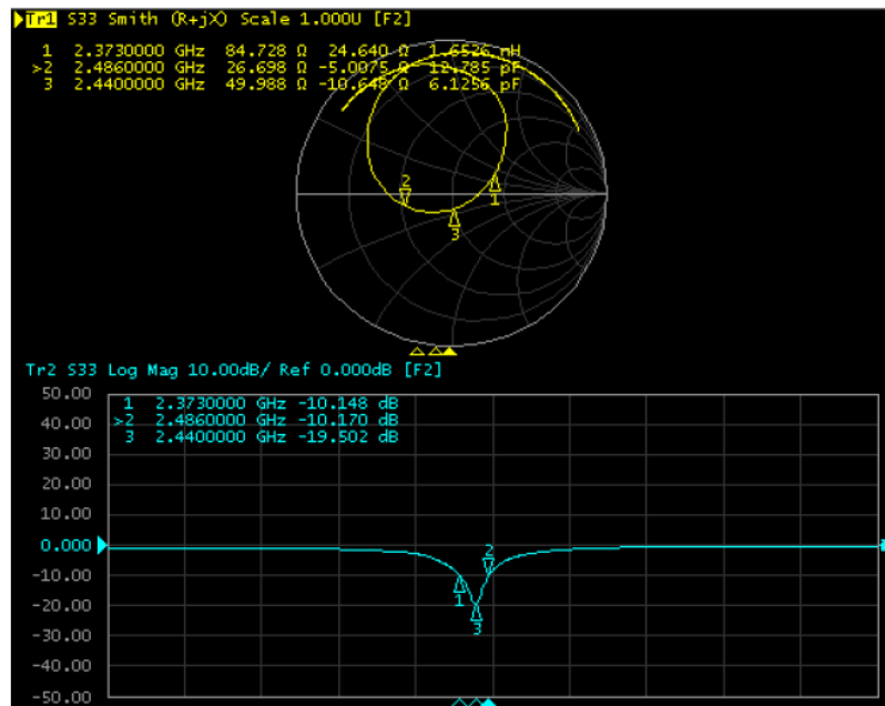
Figure 13: Antenna Return Loss
