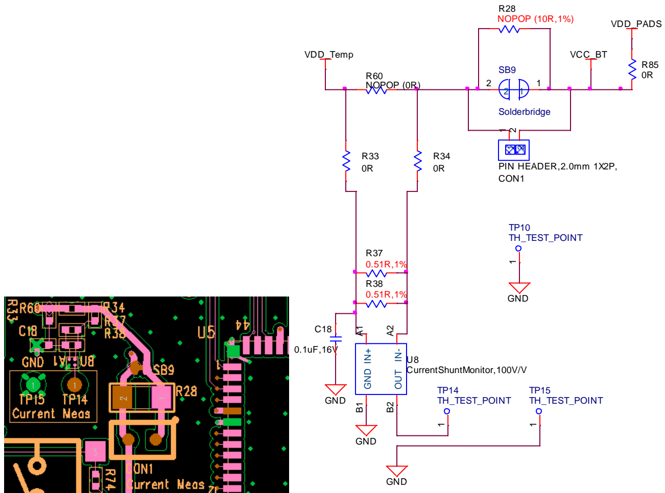
Figure 16: Current measurement Schematic and component location
