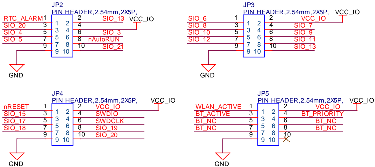
Figure 8: Breakout board connectors
