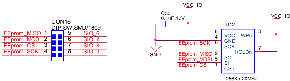
Figure 15: SPI device
