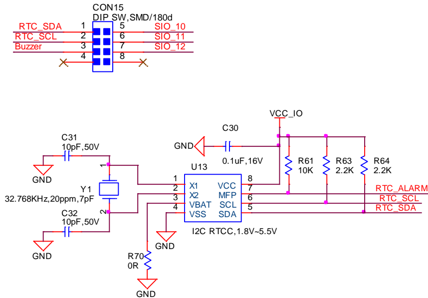
Figure 14: I2C device
