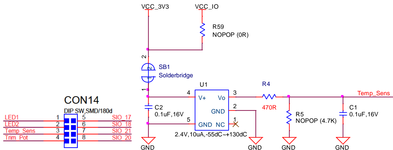
Figure 11: Temperature sensor
