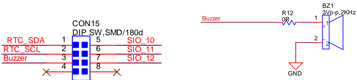
Figure 10: Buzzer
