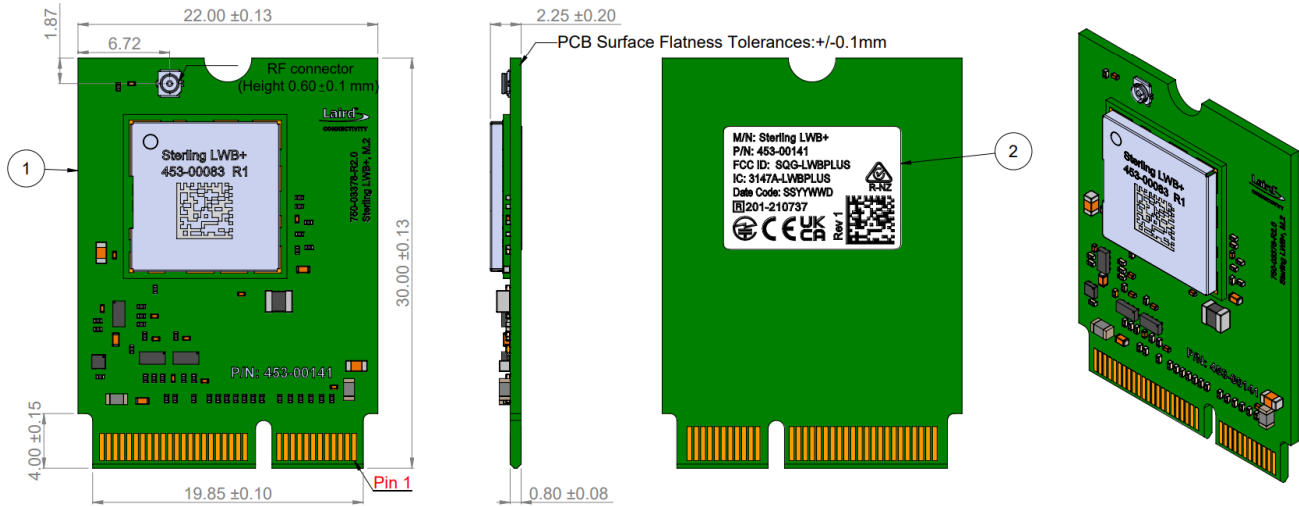
Figure 19: Sterling LWB+ M.2 2230, E-key, SDIO/UART module dimension
