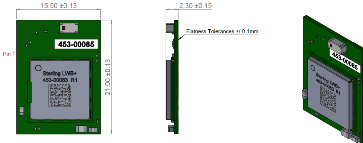
Figure 18: Sterling LWB+ MHF® 4 and chip antenna module dimension
