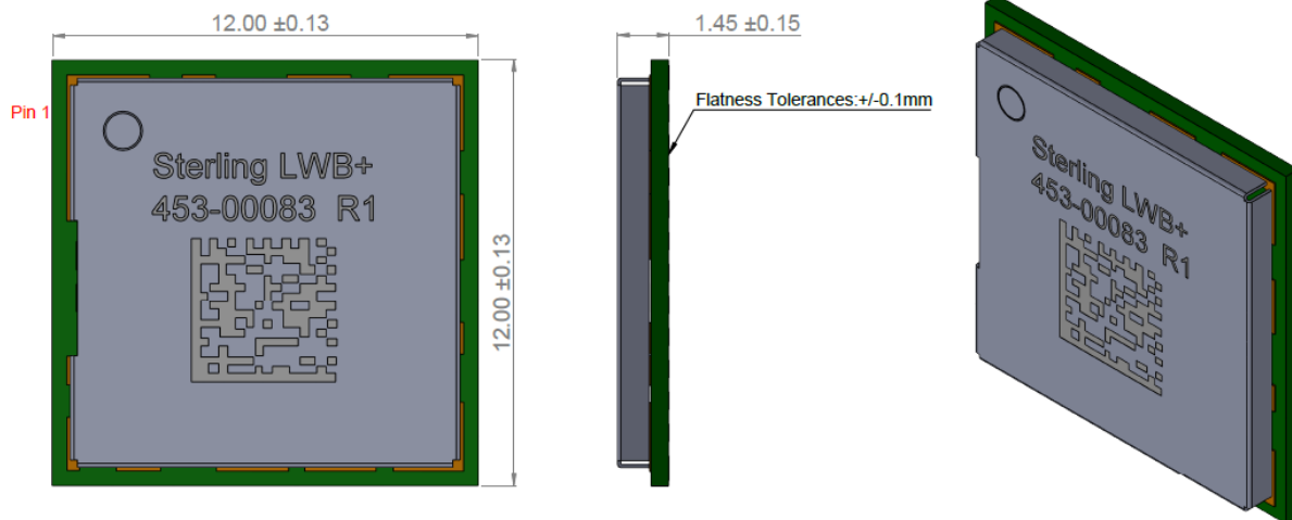
Figure 16: Sterling LWB+ base SiP module dimension
