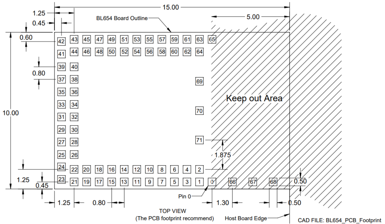
Figure 14: Land pattern and Keep-out for the 451-00001
