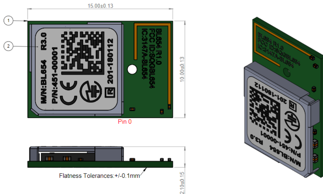
Figure 13: Mechanical Antennas - Integrated Antenna
