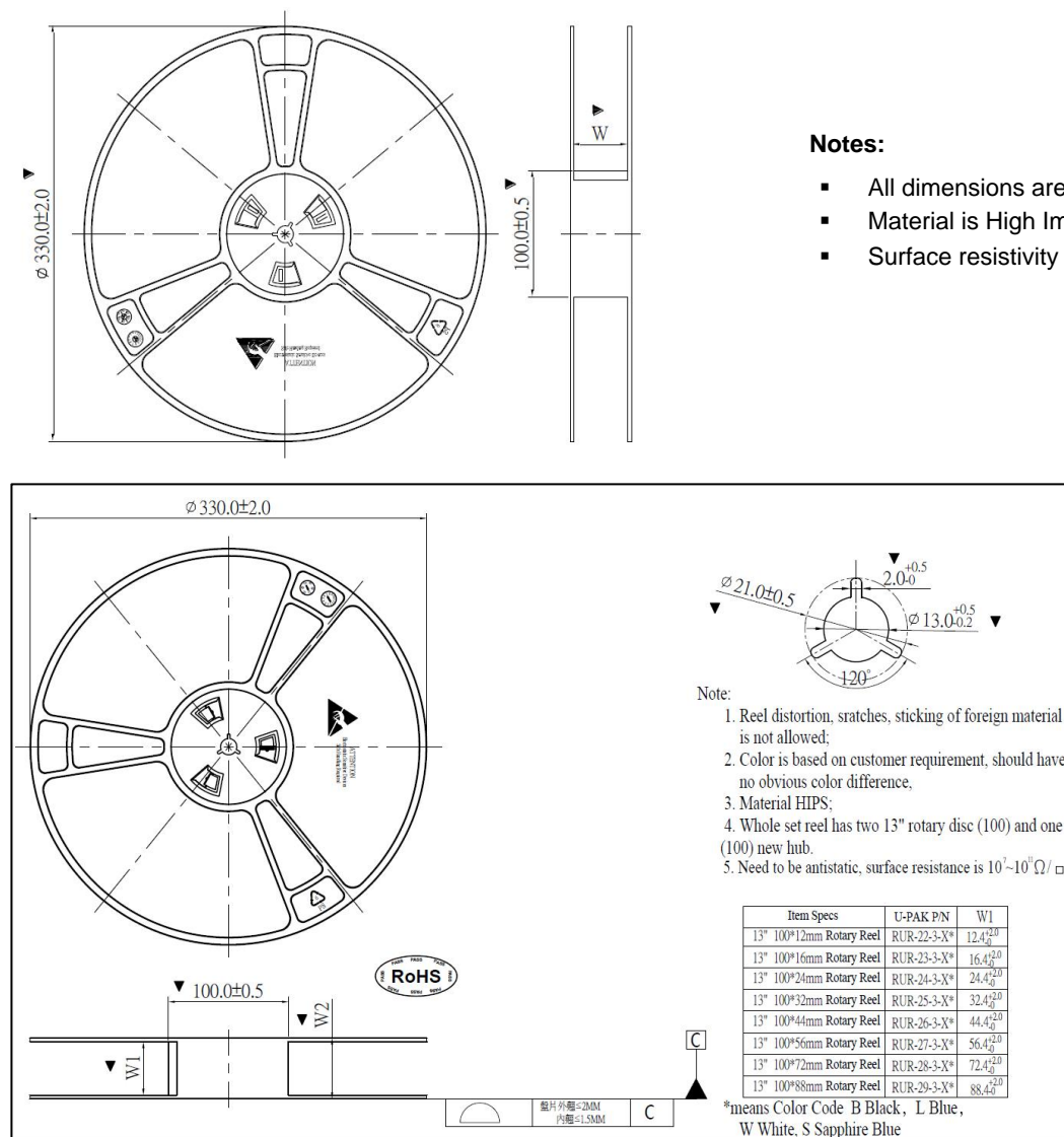
Figure 15: Reel specifications
