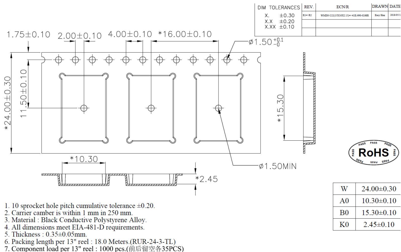
Figure 16: Tape specifications (Module Orientation – Module Antenna Side away from Tape holes)
