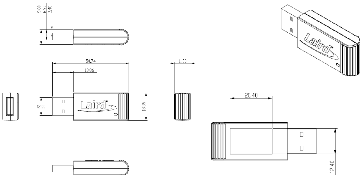
Figure 9: 451-00003 USB BLE 5.1 Dongle Mechanical details
