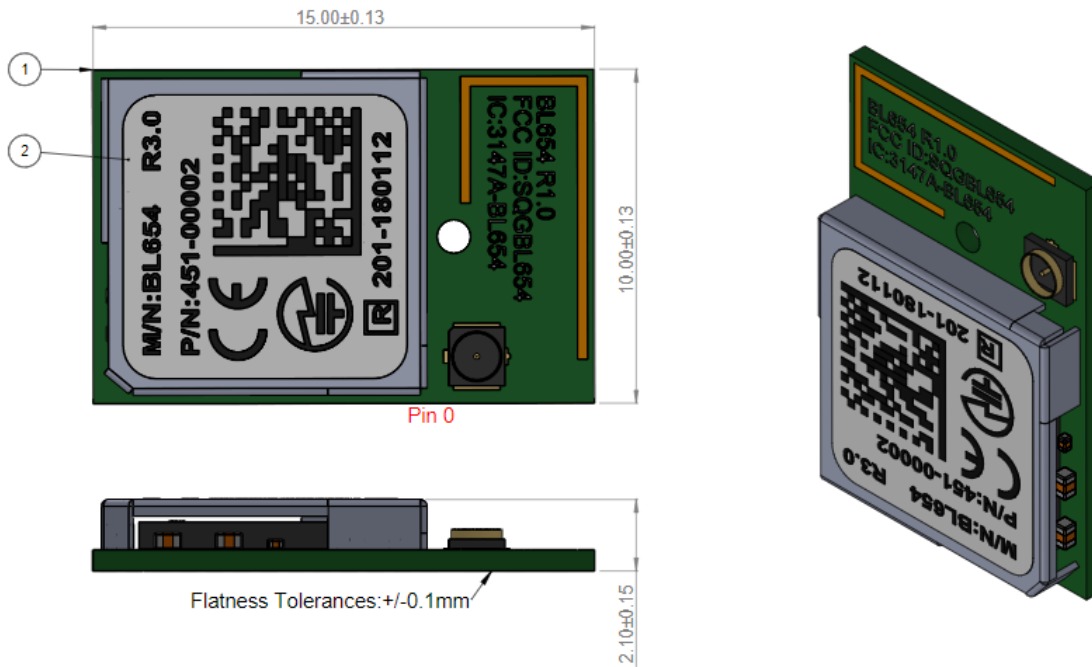
Figure 12: Mechanical Details - External Antenna
