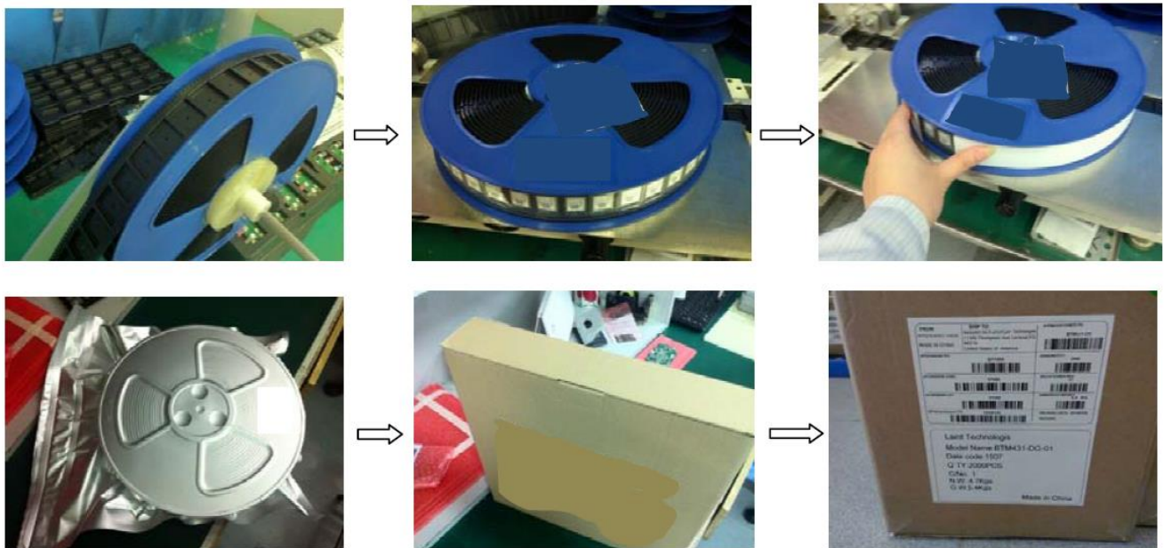
Figure 18: BL654 packaging process
