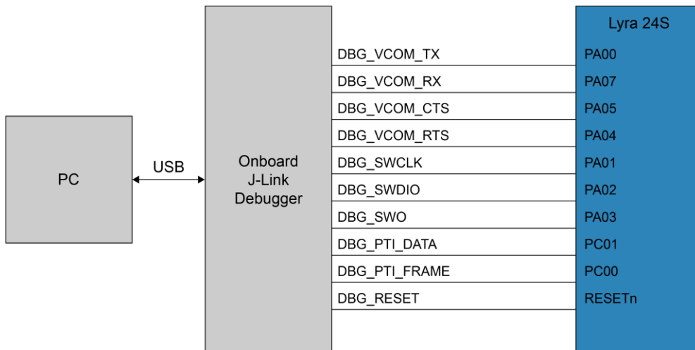
Figure 5: Lyra 24S DVK Debugger Connections
