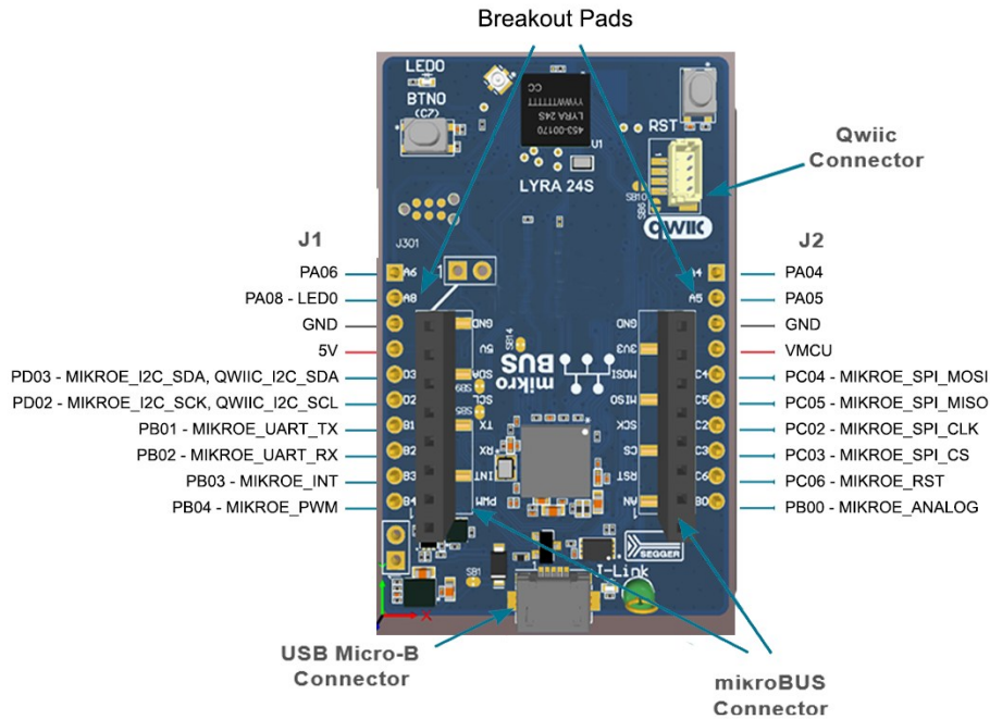
Figure 7: Lyra 24S development board Breakout Pads (J1 and J2)
