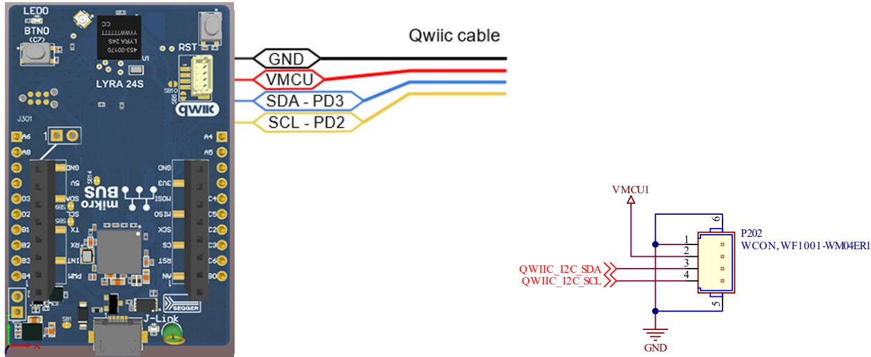
Figure 10: Qwiic connector
