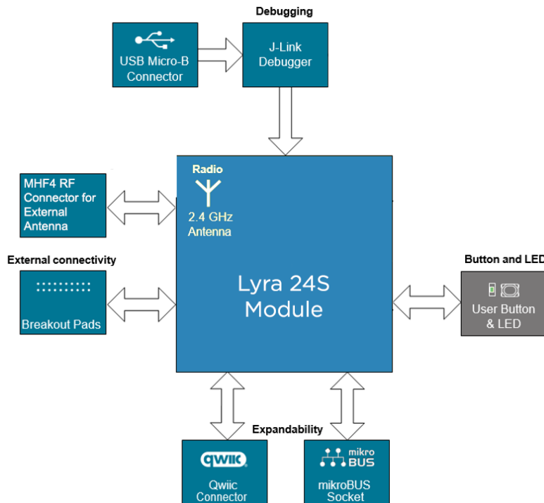
Figure 2: Lyra 24S DVK block diagram
