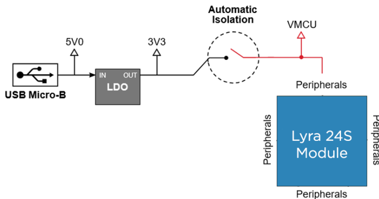
Figure 3: Lyra 24S DVK power diagram
