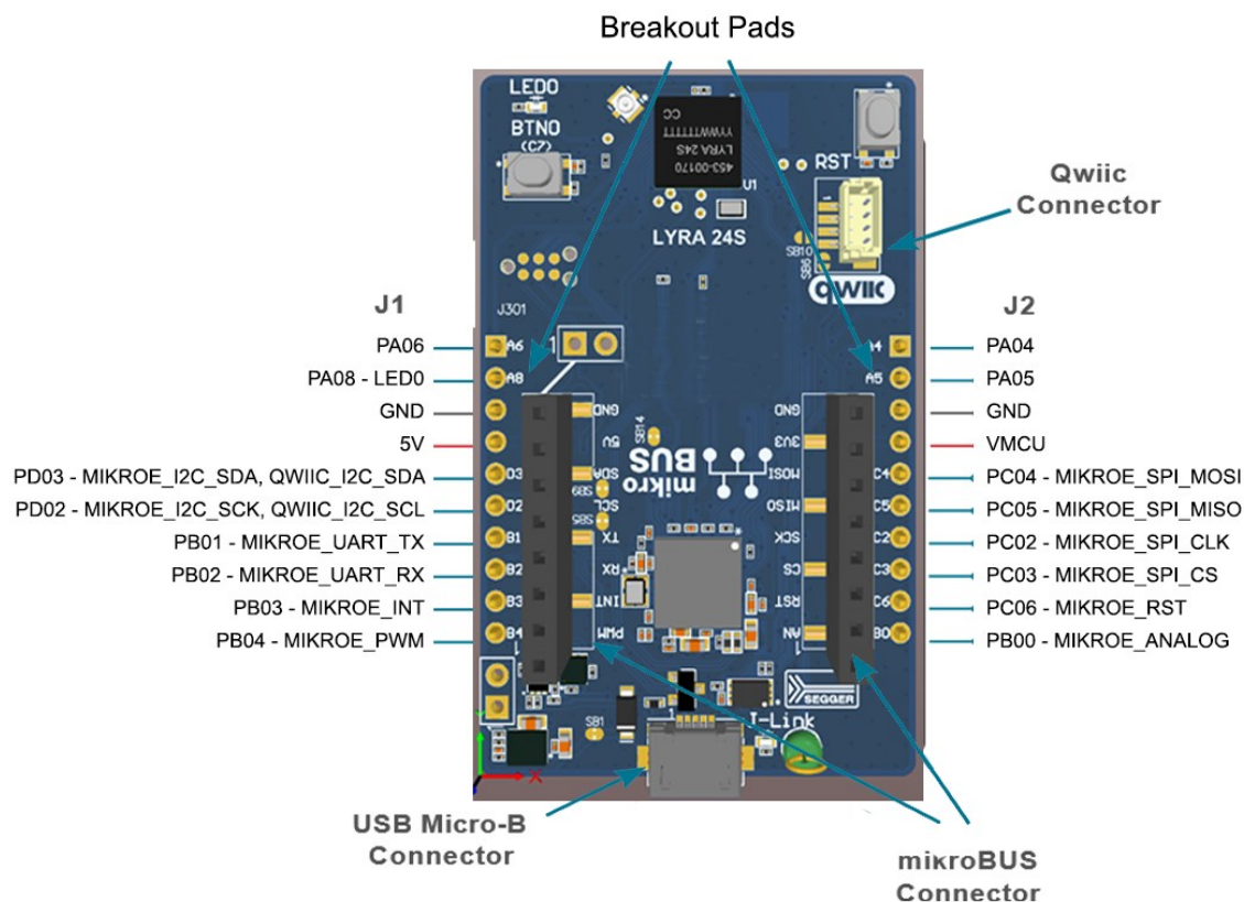
Figure 6: Lyra 24S DVK hardware connectors
