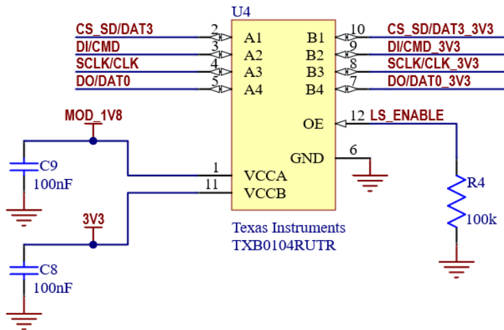
Figure 15: Logic level shifter
