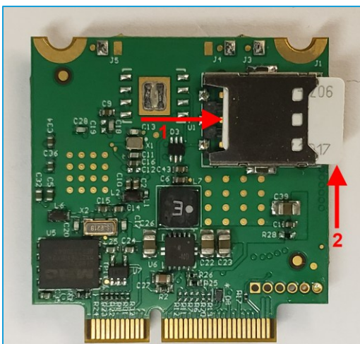
Figure 25: Removing nano SIM from Pinnacle™ 100 modem
