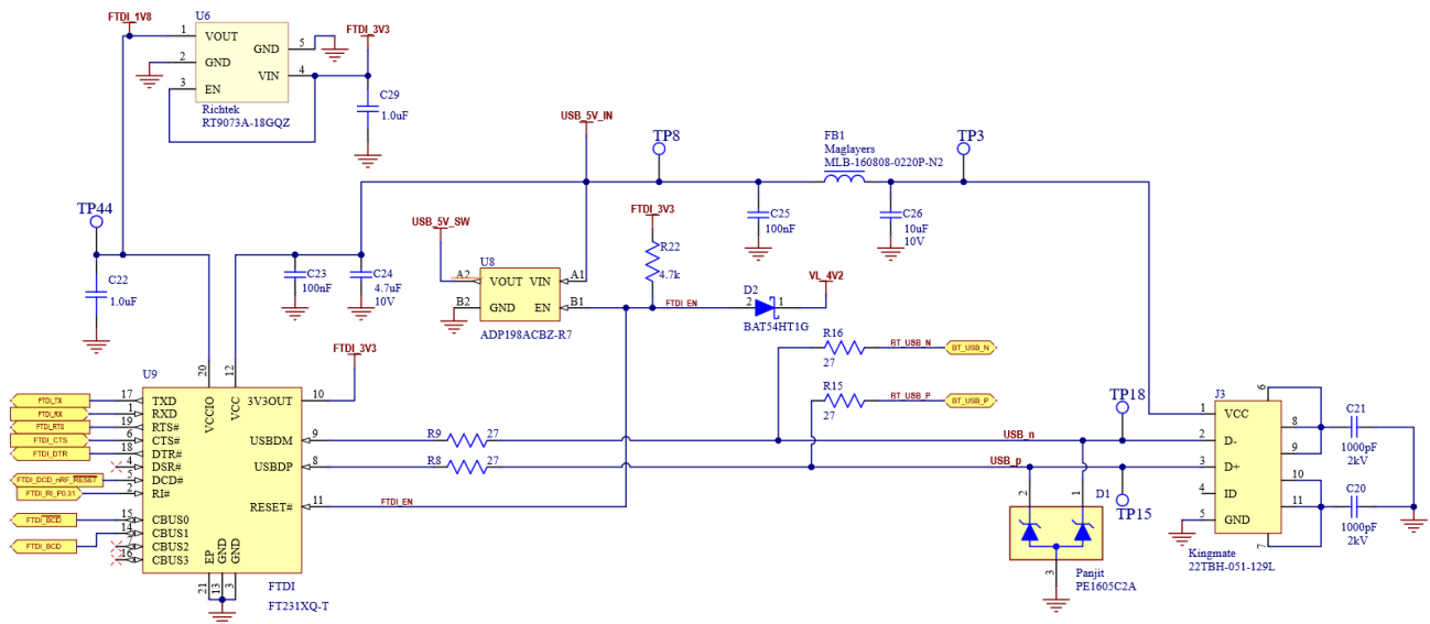
Figure 9: Power input
