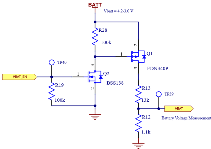
Figure 12: Battery voltage measurement
