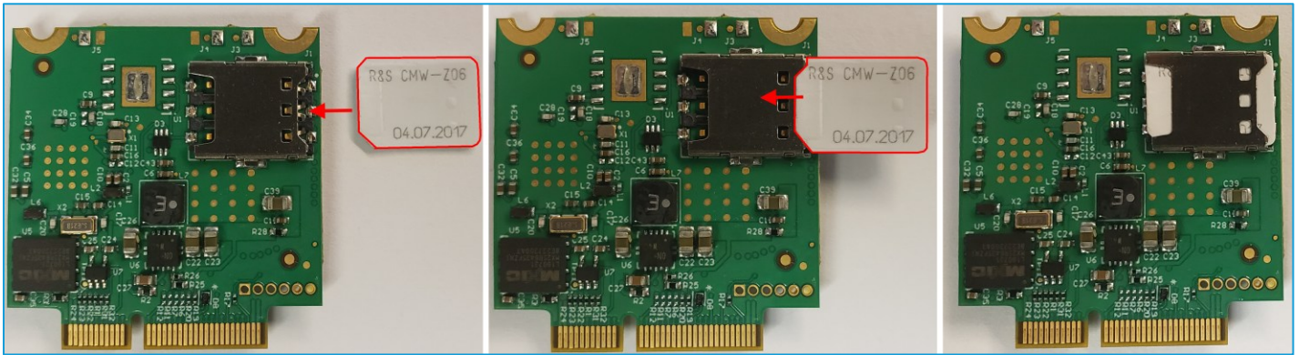
Figure 26: Insertion of nano SIM into a Pinnacle™ 100 modem (image of 453-00011)
