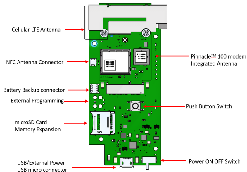
Figure 4: Micro-gateway PCBA with Pinnacle™ 100 modem – integrated antenna
