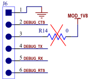
Figure 22: Debug UART interface
