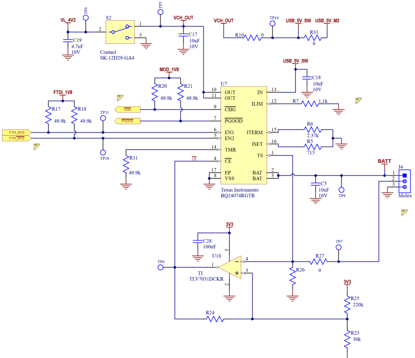
Figure 10: Battery management circuitry (Battery Backup Variant Only)
