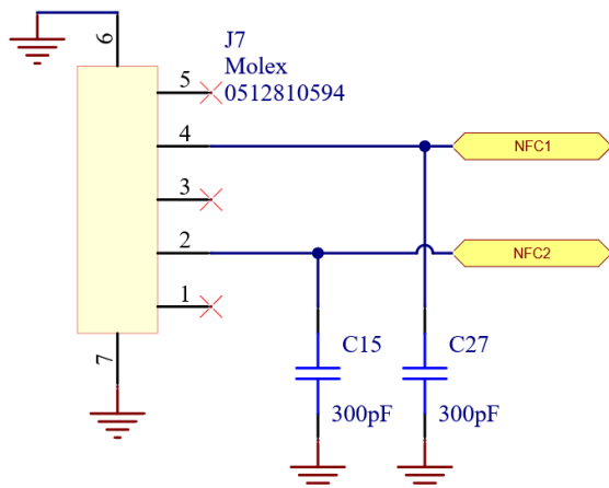
Figure 19: NFC interface
