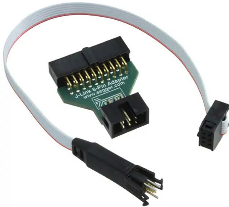
Figure 18: Tag-Connect TC2030-IDC with ARM20-CTX six-pin adapter
