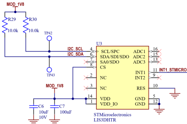
Figure 13: Internal sensor
