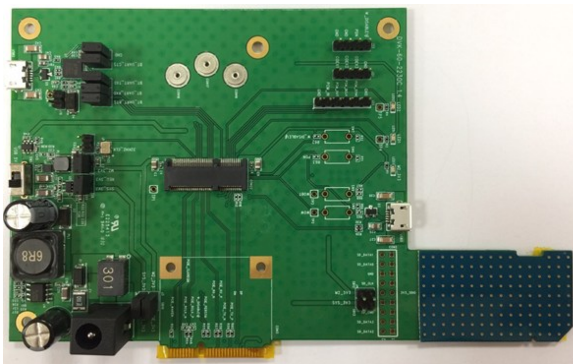
Figure 1: Development board
