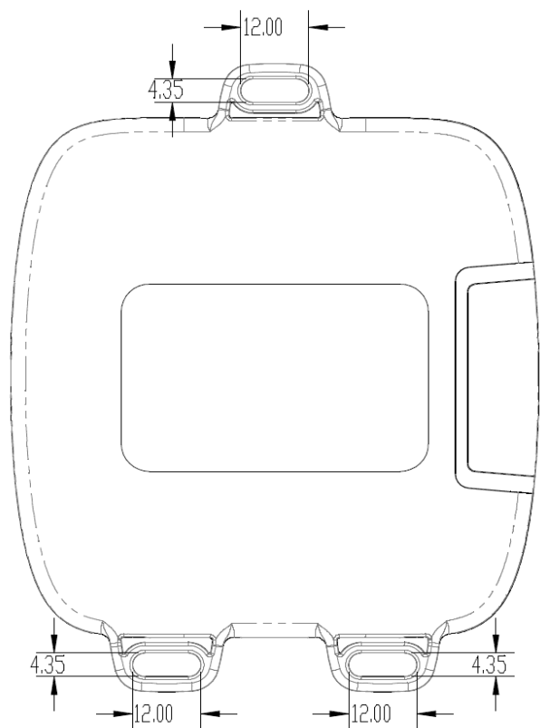
Figure 1: Rear view of Sentrius™ RS1xx Sensor with mounting hole dimensions
