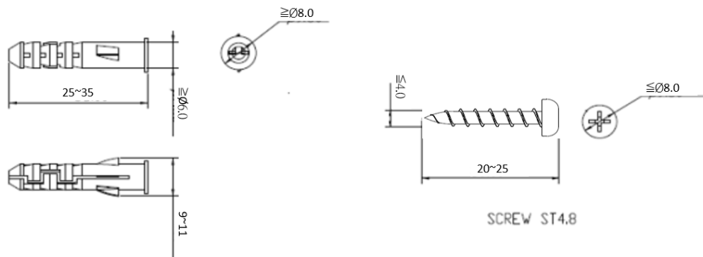
Figure 2: Sentrius™ RS1xx Sensor screw specification for wall mounting
