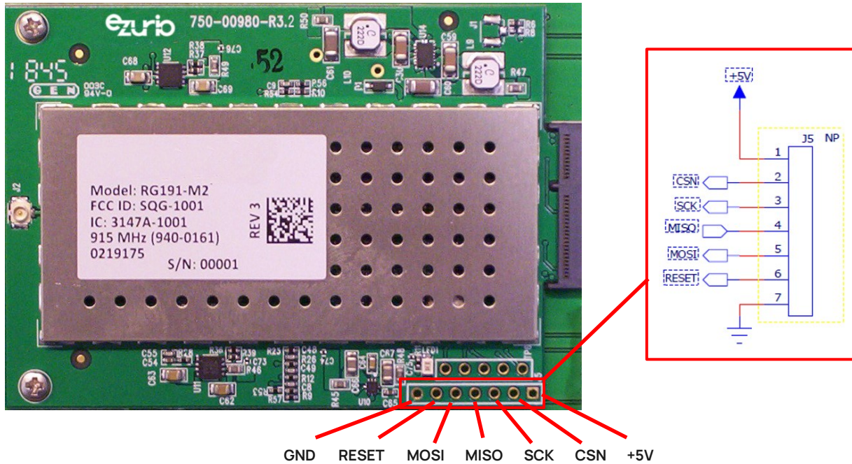
Figure 2: J5 signals description
