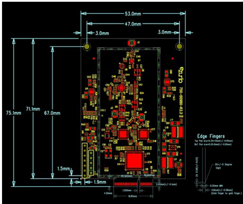
Figure 3: RG1xx-M2 mechanical drawing
