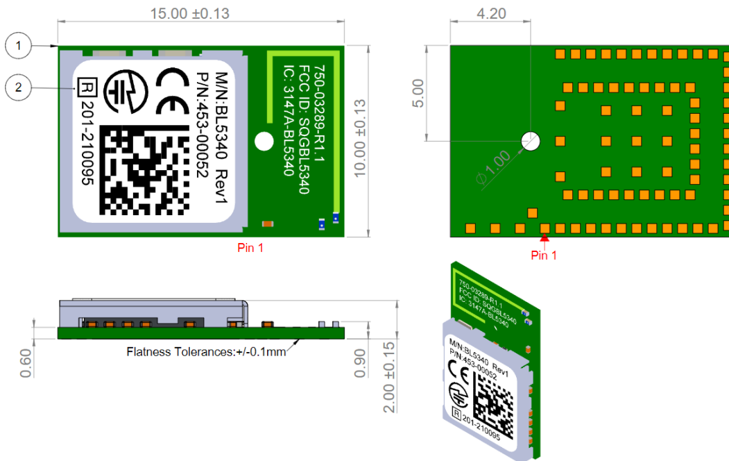
Figure 18: Mechanical Details - Chip Antenna
