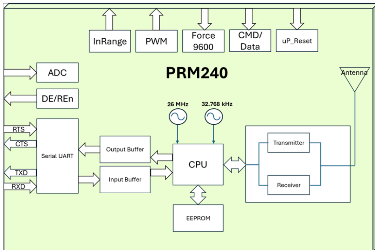
Figure 2: PRM240-R2 functional block diagram
