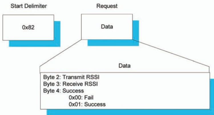
Figure 2: Send Data Complete Packet Format
