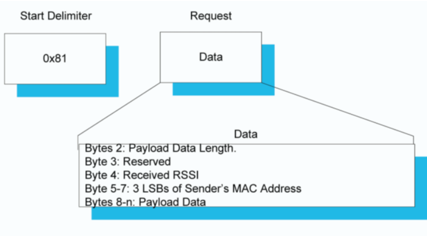
Figure 3: Receive API Packet Format
