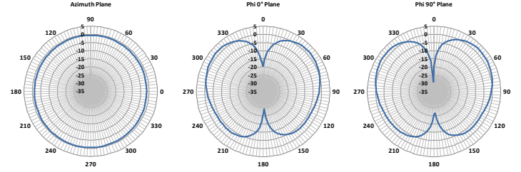
Radiation Pattern at 1850 MHz
