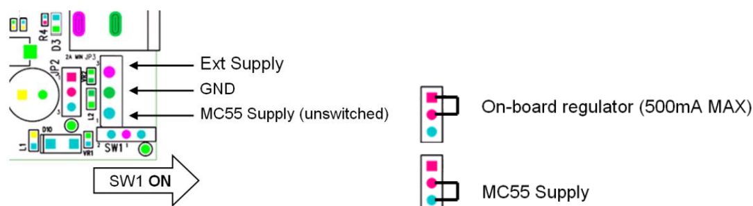
Figure 2: JP2 Settings
