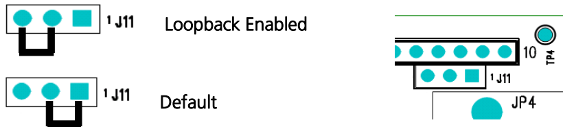
Figure 5: J11 Settings
