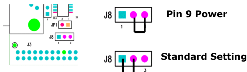
Figure 3: J8 Settings
