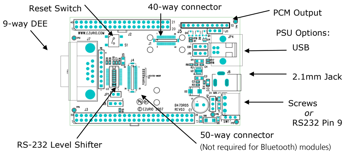
Figure 1: Development Board
