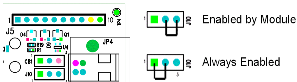
Figure 4: J10 Settings
