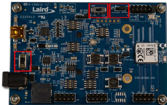
Figure 2: Switch and jumpers position
