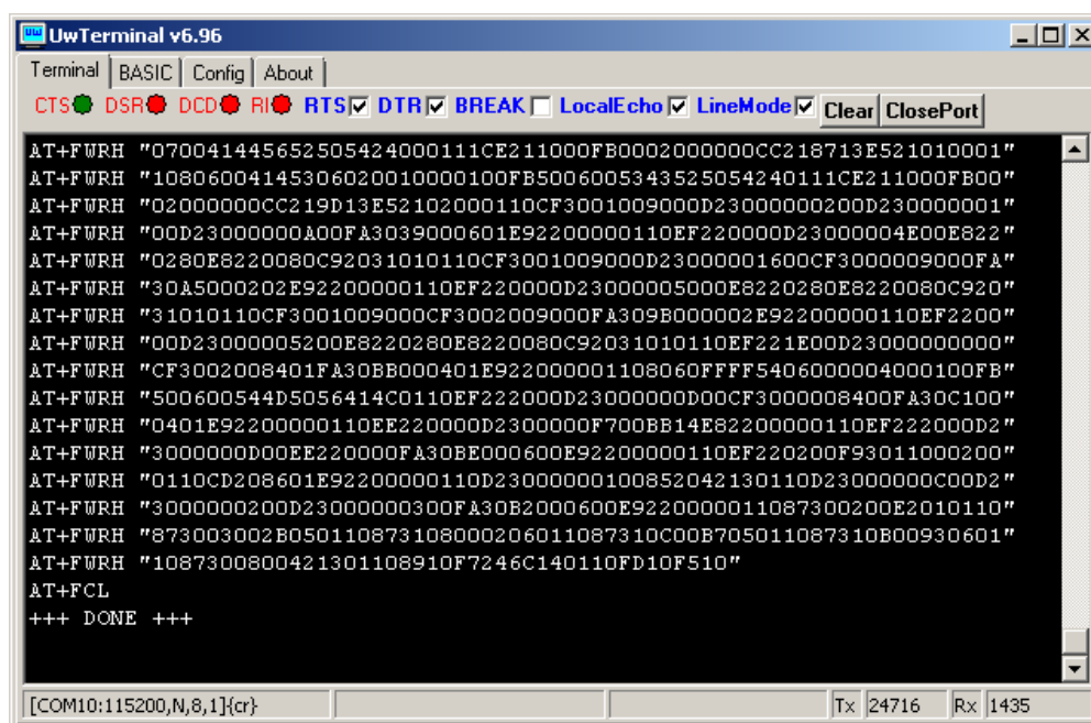
Figure 8: Compiled and loaded
