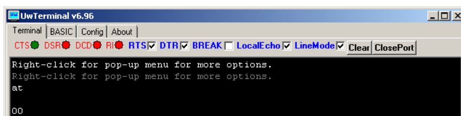
Figure 6: Comms OK
