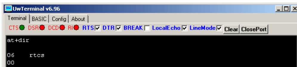
Figure 10: UwTerminal
