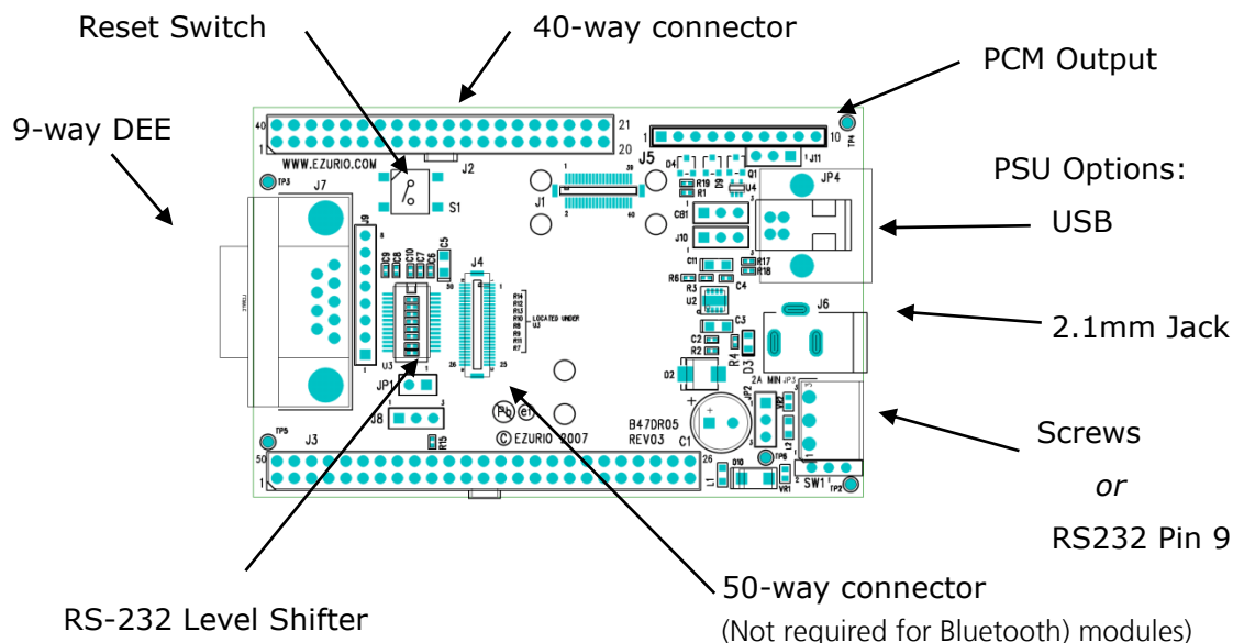
Figure 1: Development Board
