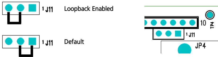
Figure 5: J11 Settings
