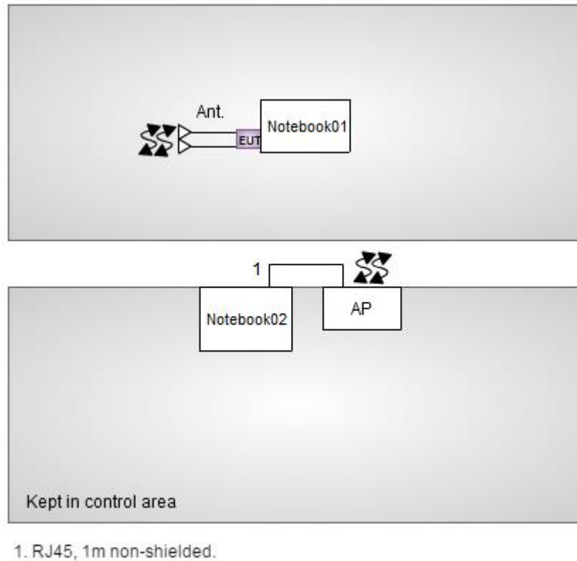
Test Setup Diagram (EMS)
