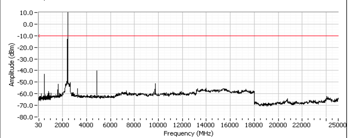
Out of Band Spurious Emissions 802.11b at 2437MHz
