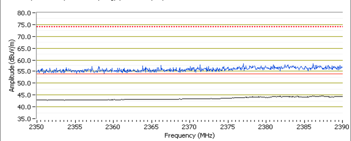
RB 1 MHz; VB 10 Hz (Black Trace) Avg, (Blue Trace) Pk, Vertical
