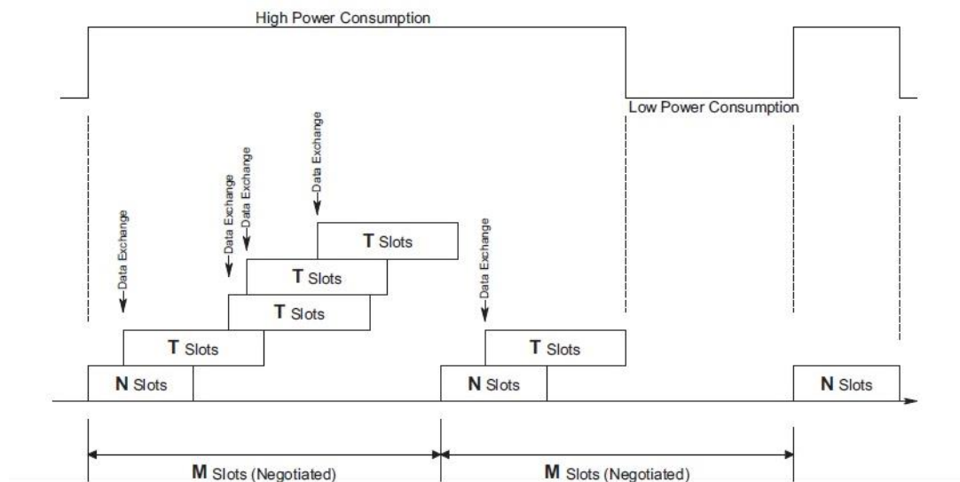
Figure 1: Power consumption when sniff mode is active
