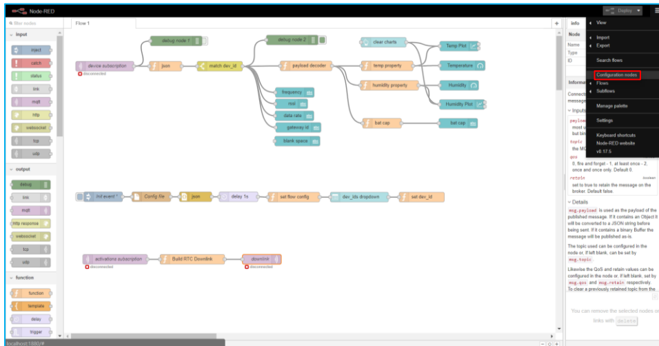
Figure 46: Configuring nodes
